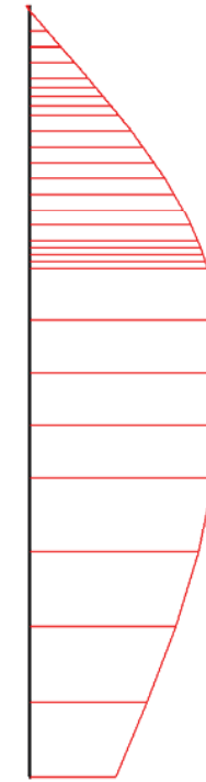
Fig. 252 Horizontal displacements in beam (plate no: 1) Extreme value 27,28 \cdot 10^{-3} m (phase: 10)
