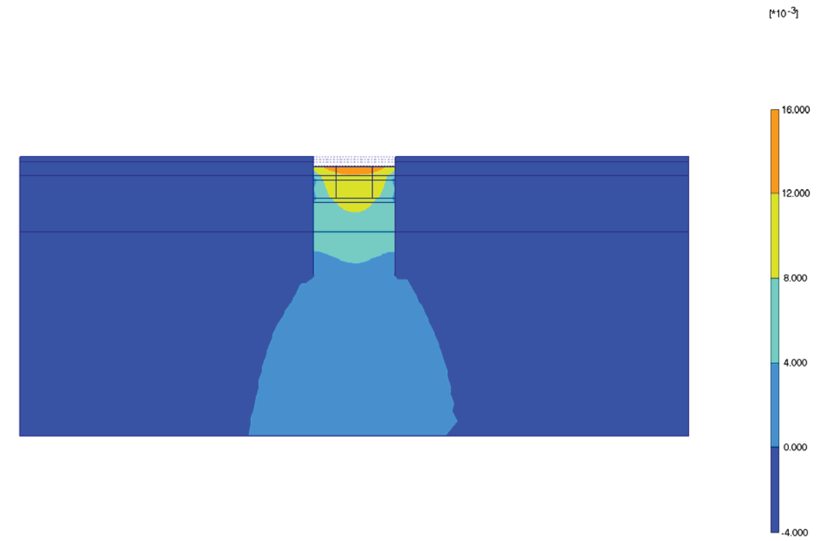
Fig. 113 Plot of vertical displacements (shadings) - step no: 15 - ( phase: 5 )
