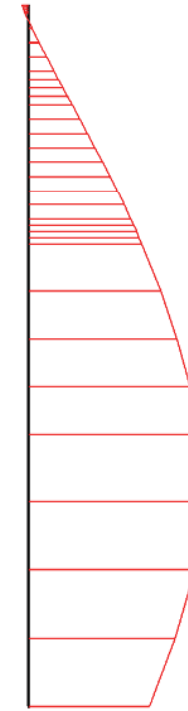
Fig. 152 Horizontal displacements in beam (plate no: 1) Extreme value 13,19 \times 10^{-3} m (phase: 6)
